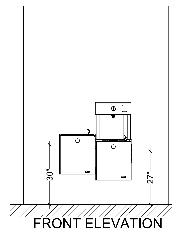
Hi-Lo Drinking Fountain Scale: 1/2" = 1'-0"
