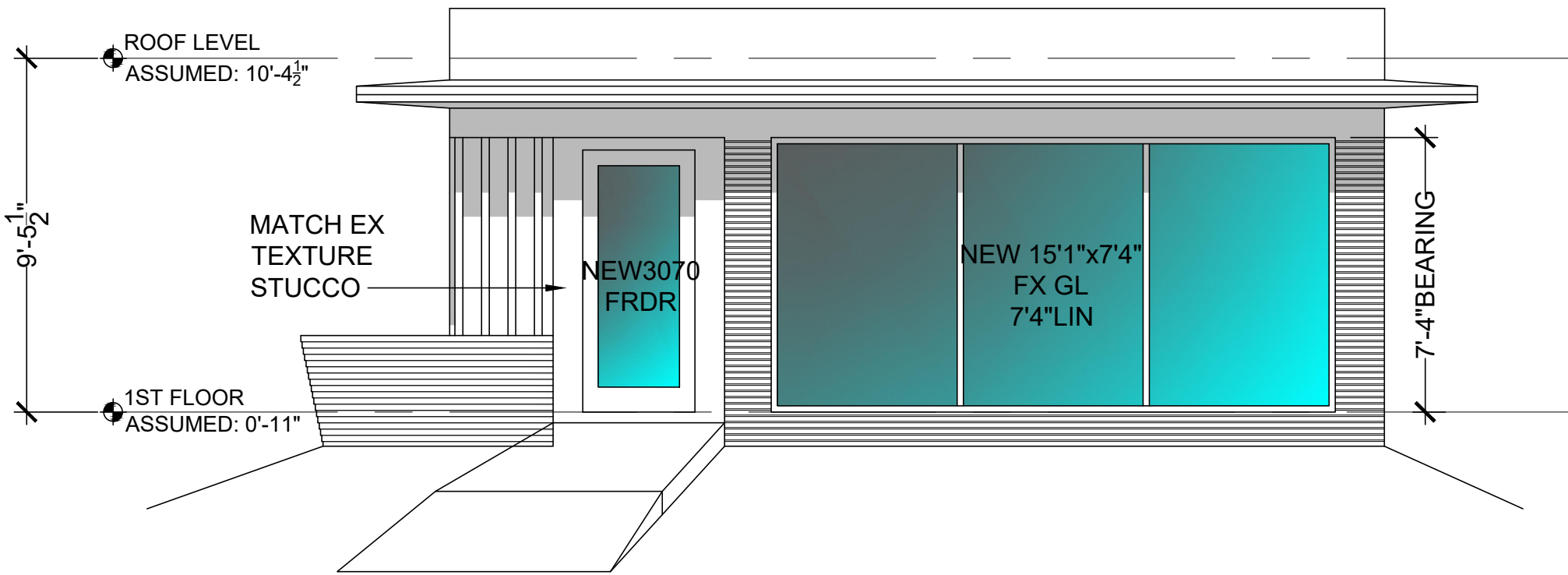
North Elevation Renovation Scale: 1/4" = 1'-0"
