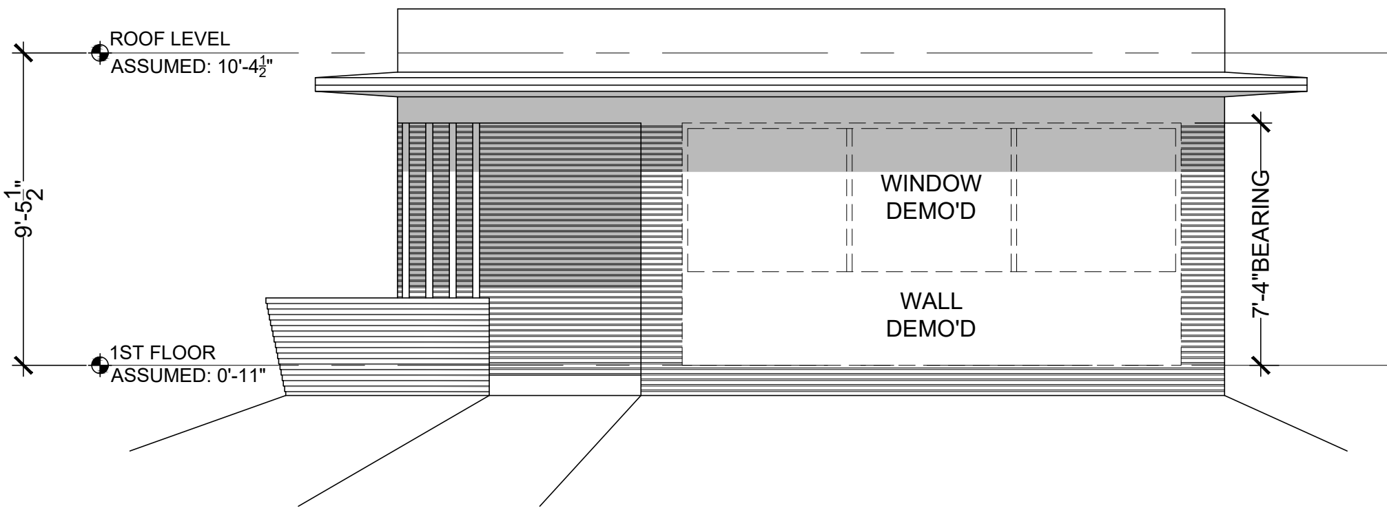
North Elevation Existing Scale: 1/4" = 1'-0"
