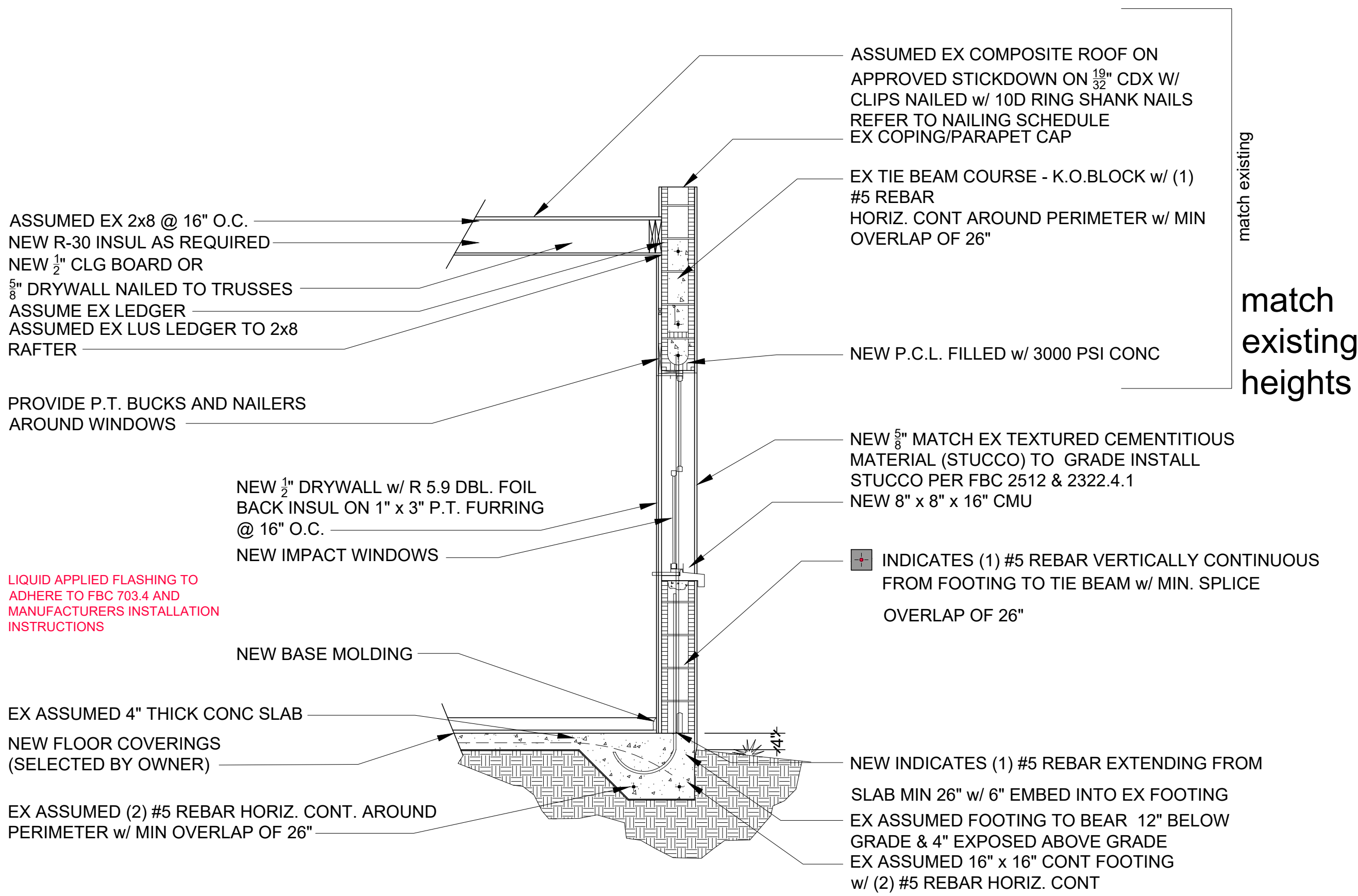
A-A Typical Wall Section Scale: 1/2"=1'-0"
