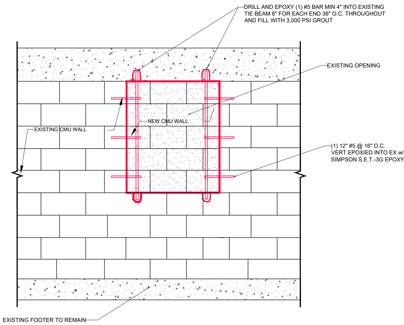
Block Infill Detail Scale: 1/2"=1'-0"
