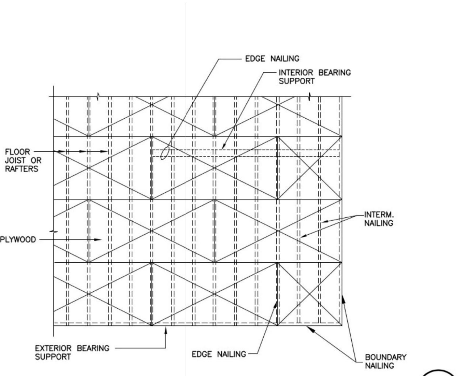
ROOF & FLOOR DIAPHRAGM
