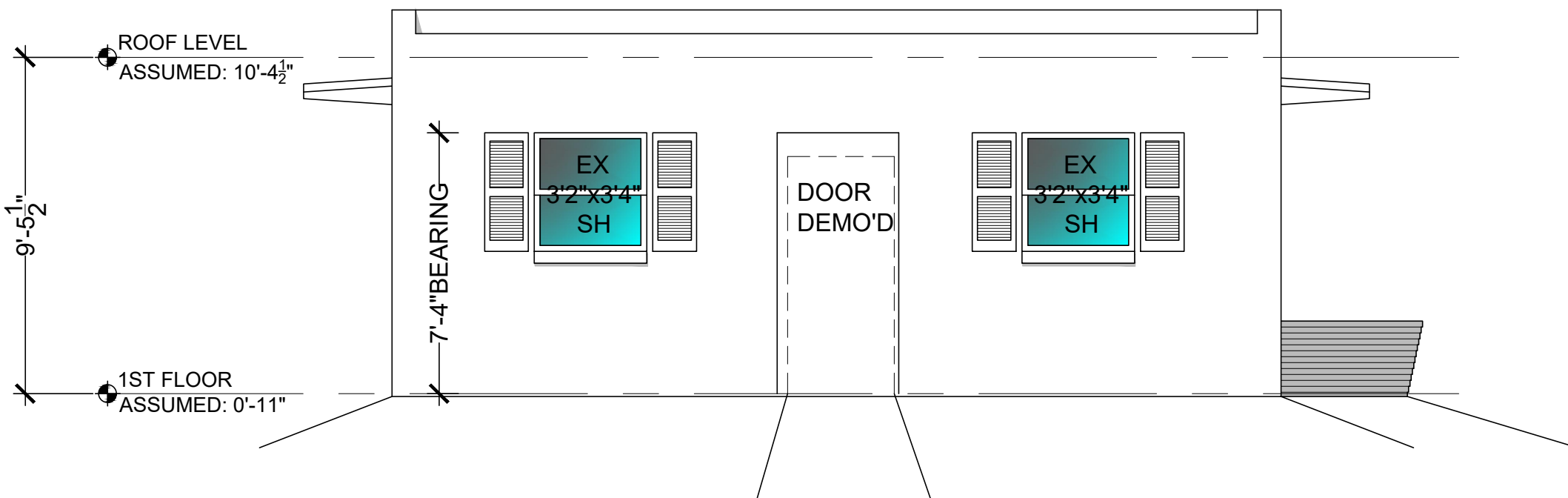
South Elevation Existing Scale: 1/4" = 1'-0"
