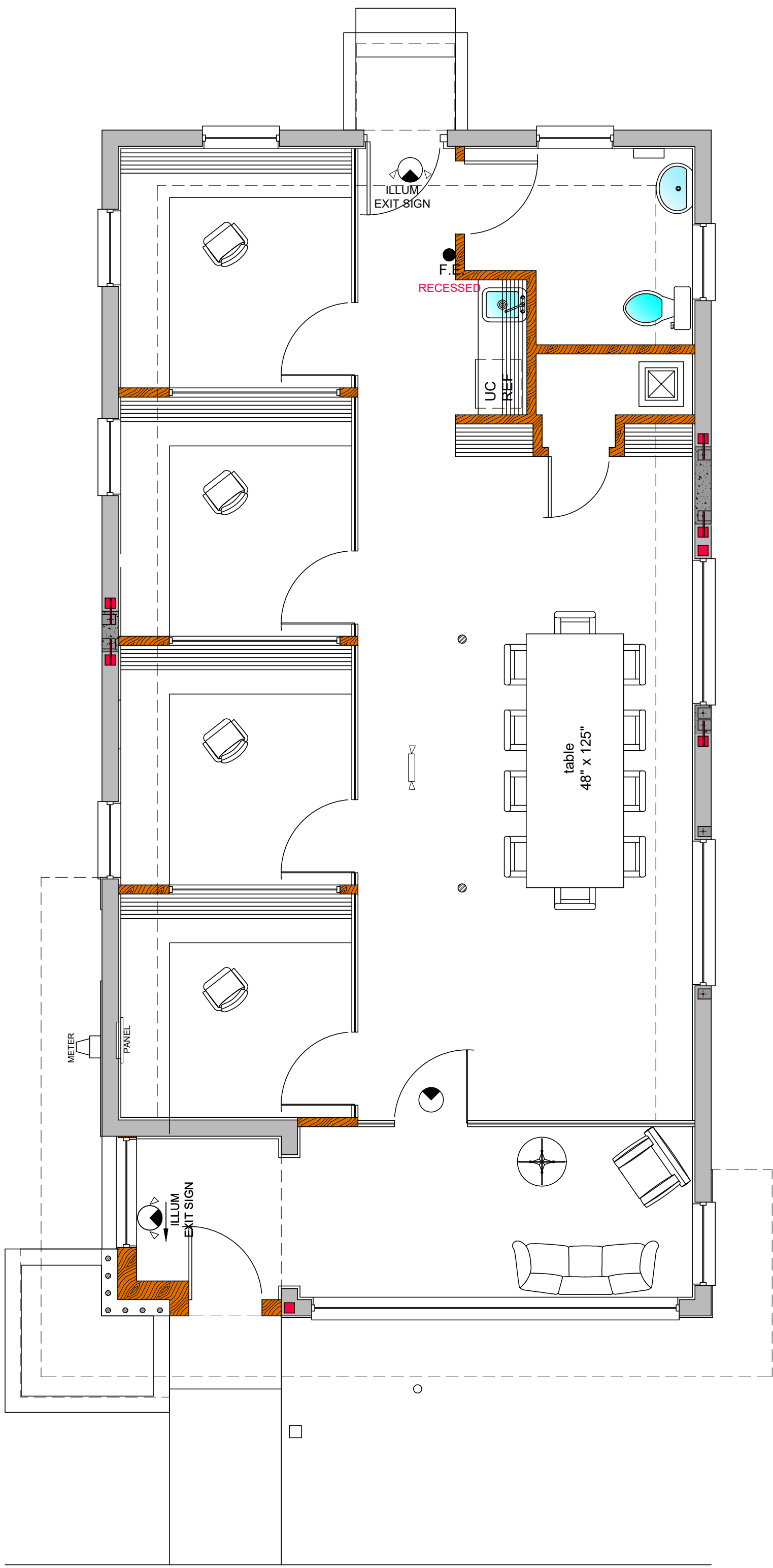
Furniture Floor Plan Scale: 1/4" = 1'-0"
