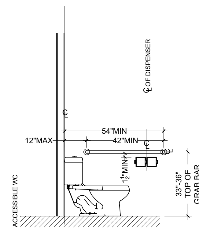
ACCESSIBLE STALL w/ 36" GRAB BAR, 42" GRAB BAR, TOILET TISSUE DISPENSER
