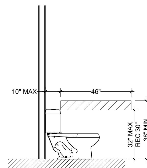
W.C. Grab Bar Blocking Location Scale: 3/8" = 1'-0"
