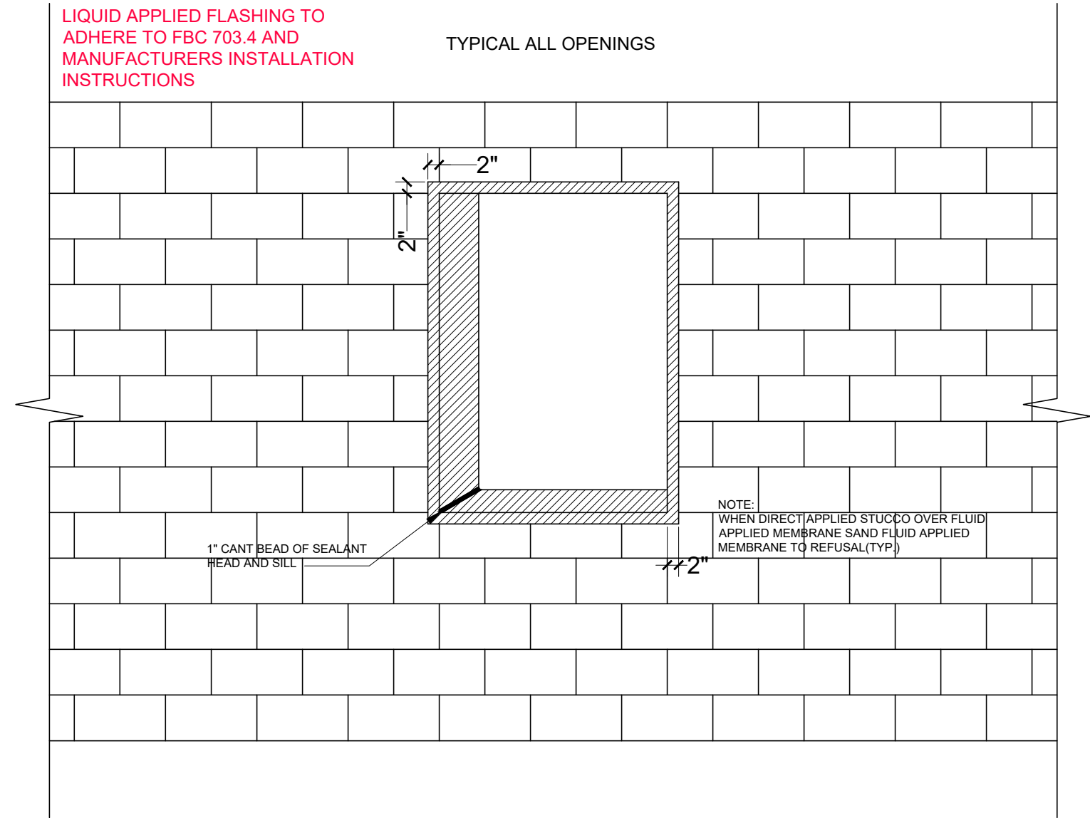
Flashing Detail - Window Scale: 1/2"=1'-0"
