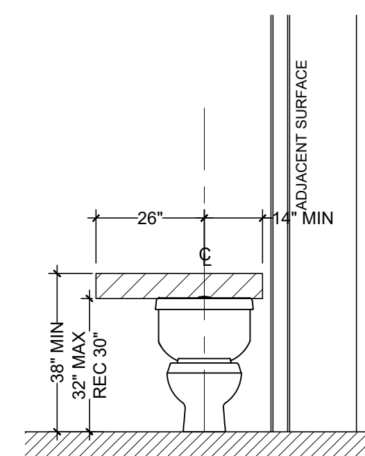
W.C. Grab Bar Blocking Location Scale: 3/8" = 1'-0"
