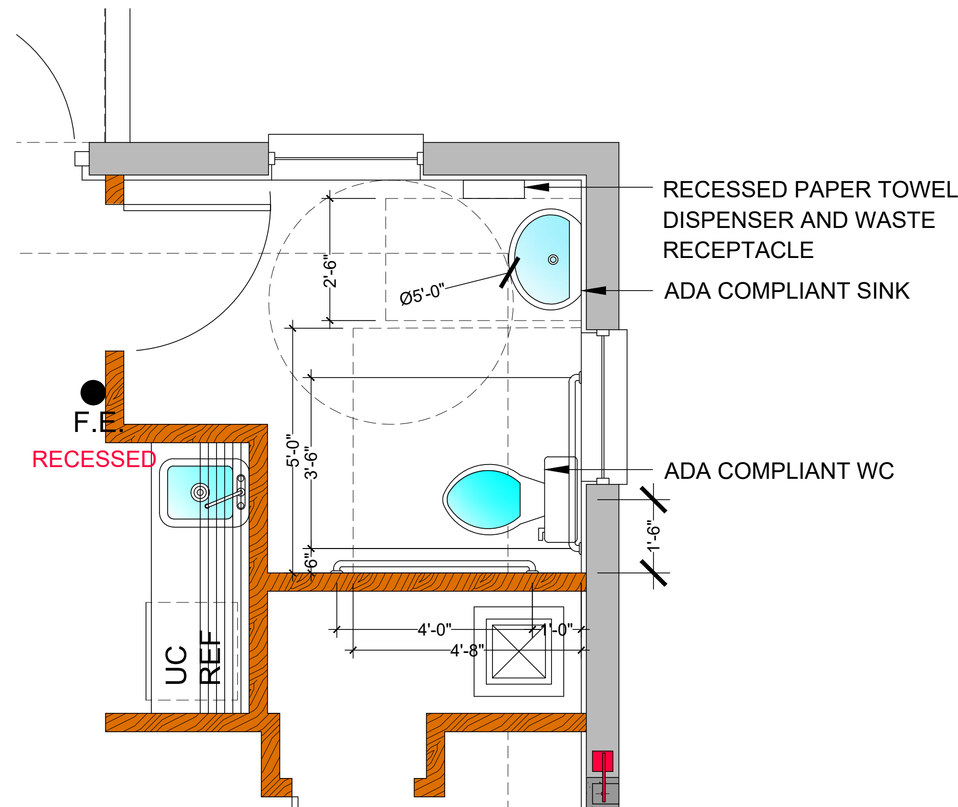
ADA Lavatory Layout Scale: 1/2" = 1'-0"
