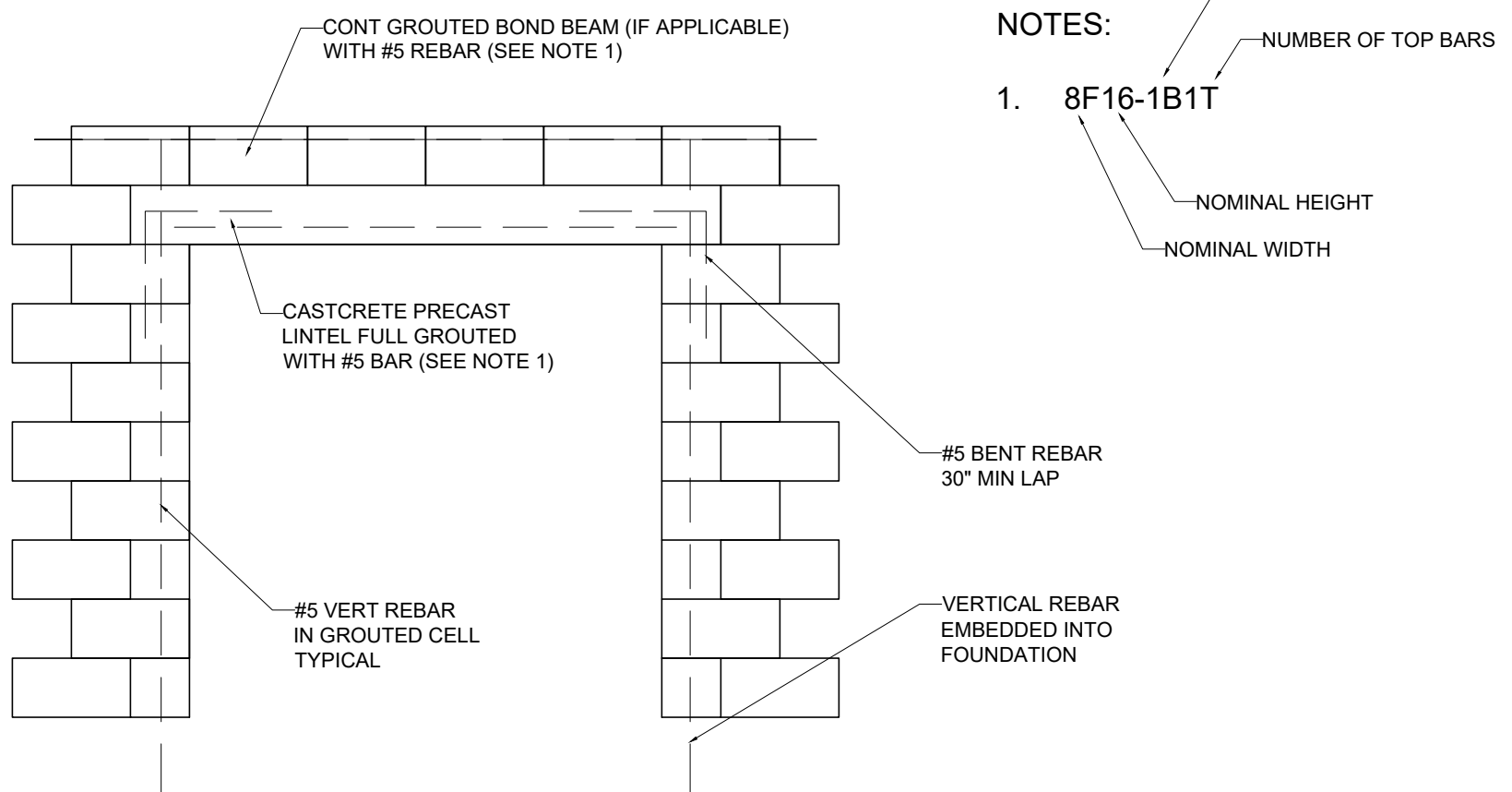
Typical Lintel/Bond Beam Construction Scale: 1/2"=1'-0"
