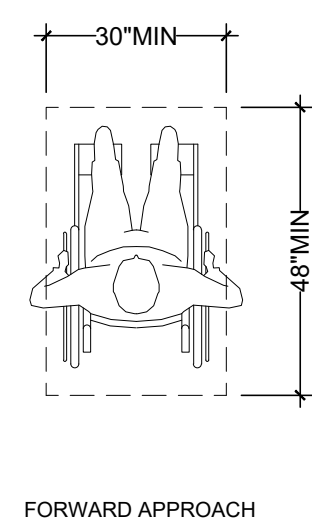
Clear Floor Space Scale: 3/8" = 1'-0"
