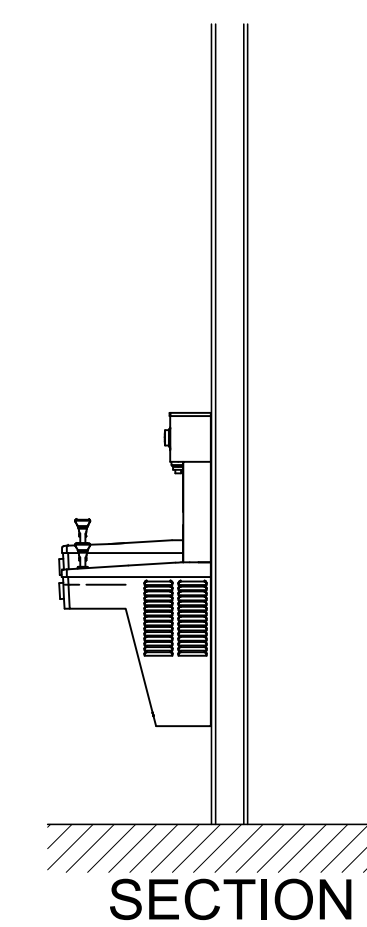
Hi-Lo Drinking Fountain Scale: 1/2" = 1'-0"
