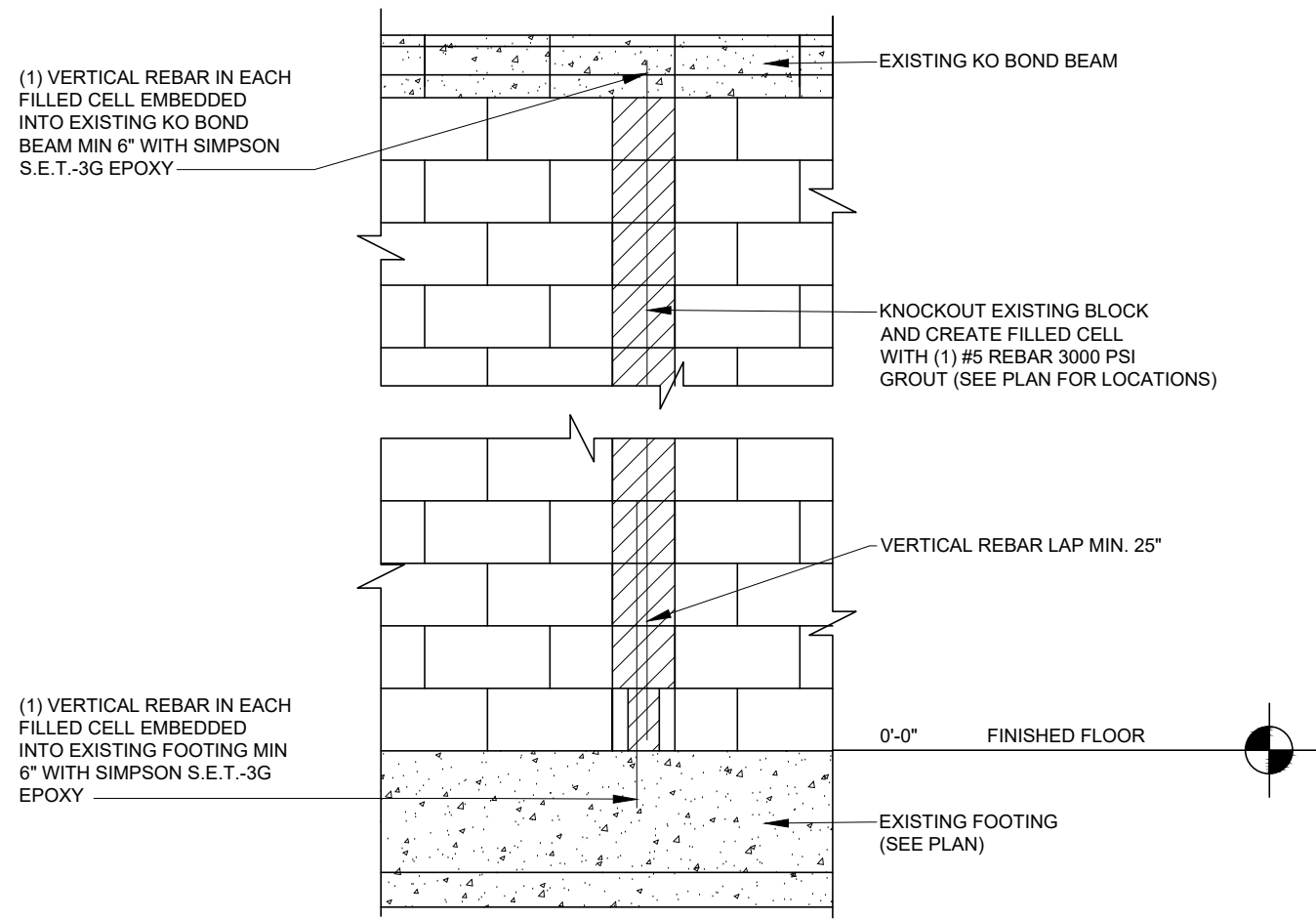
Filled Cell Detail Scale: 1/2"=1'-0"
