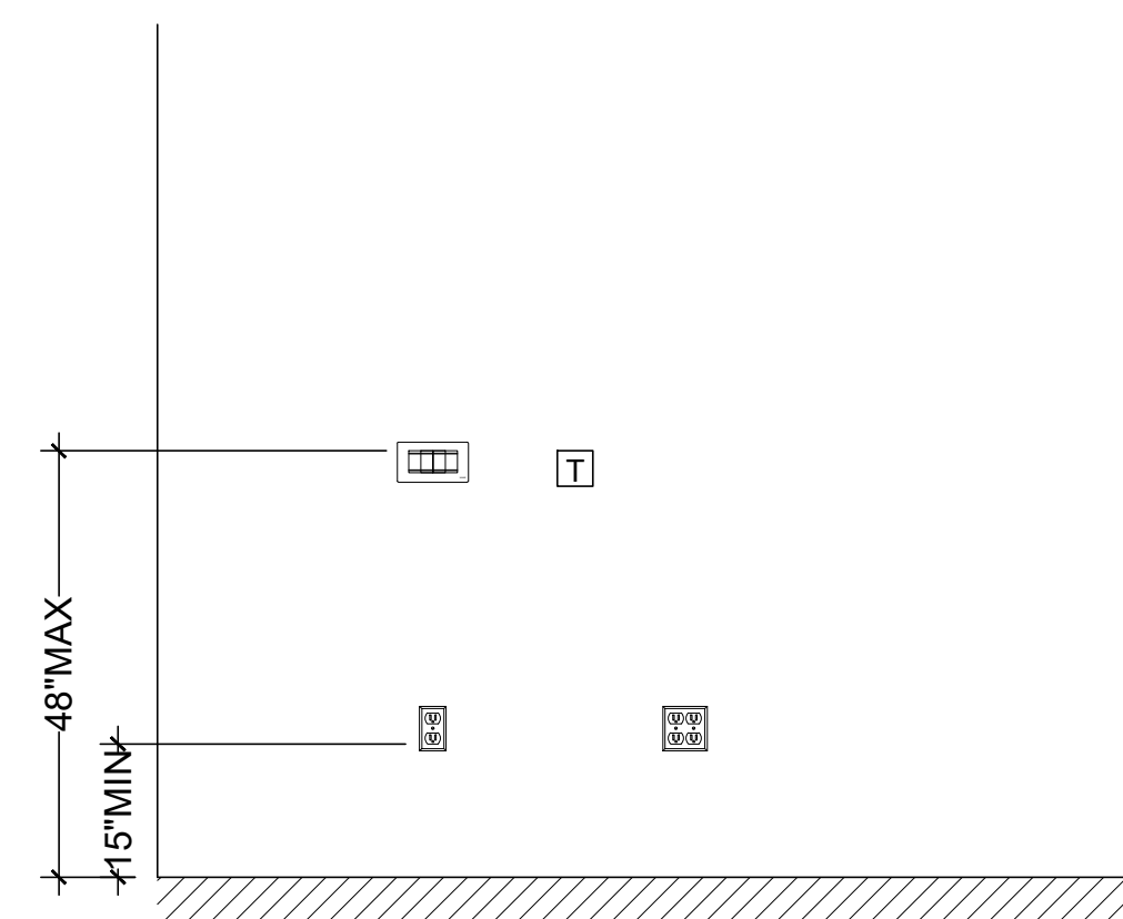
Elec Control Locations Scale: 1/2" = 1'-0"
