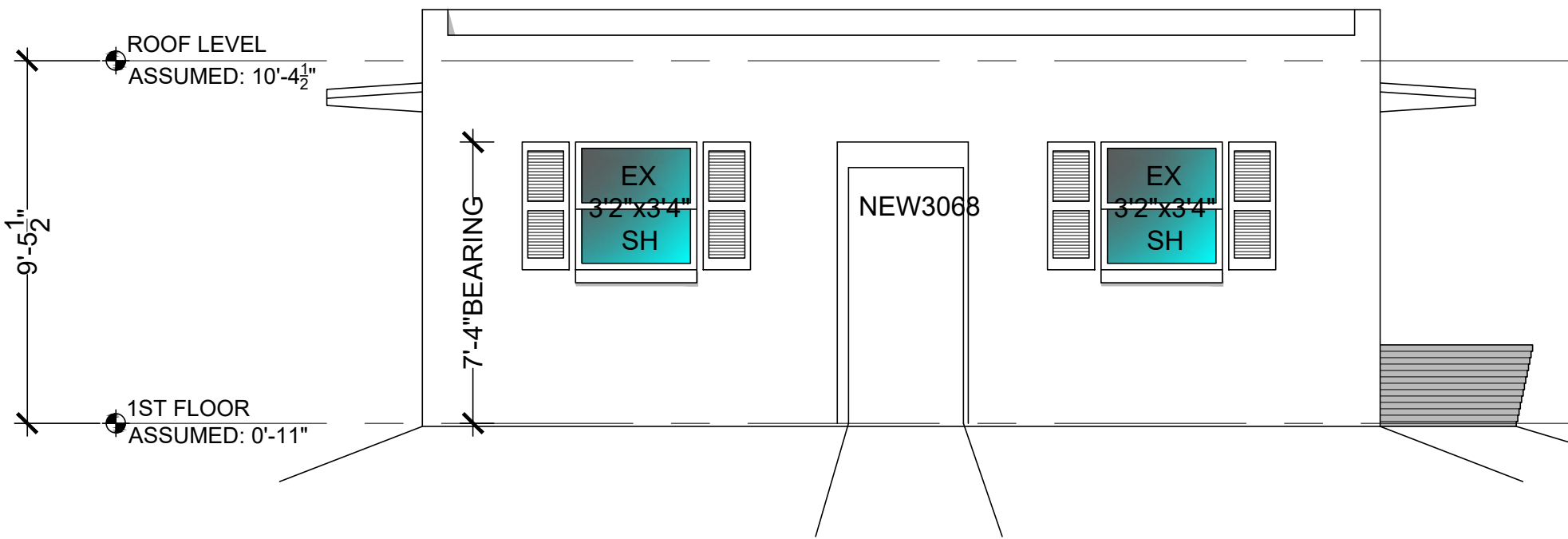
South Elevation Renovation Scale: 1/4" = 1'-0"
