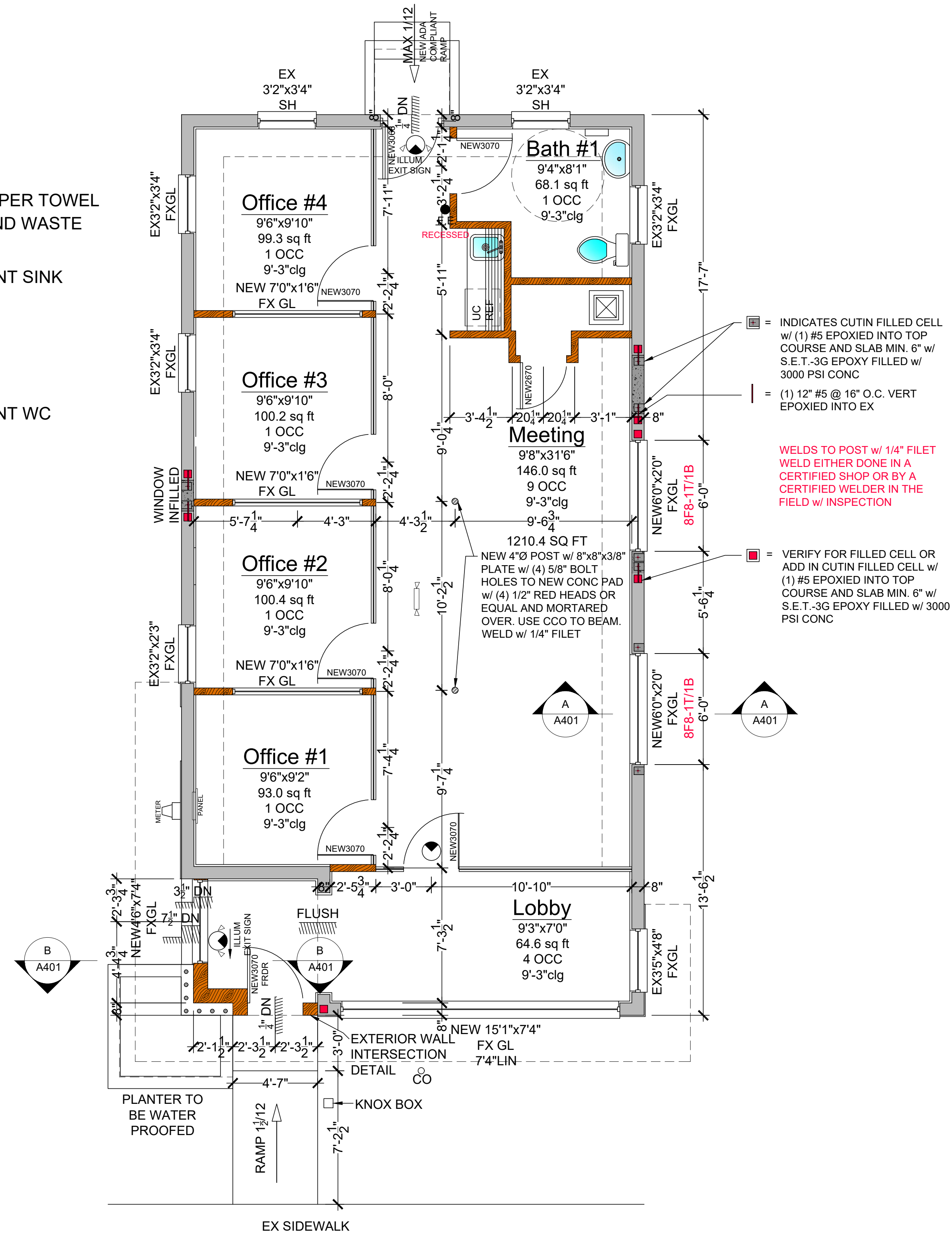
Renovation Floor Plan Scale: 1/4" = 1'-0"
