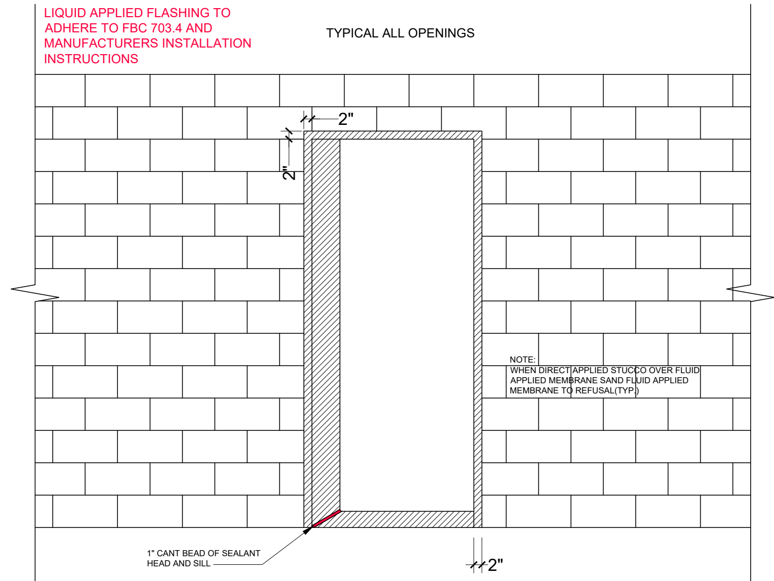
Flashing Detail - Doorway Scale: 1/2"=1'-0"
