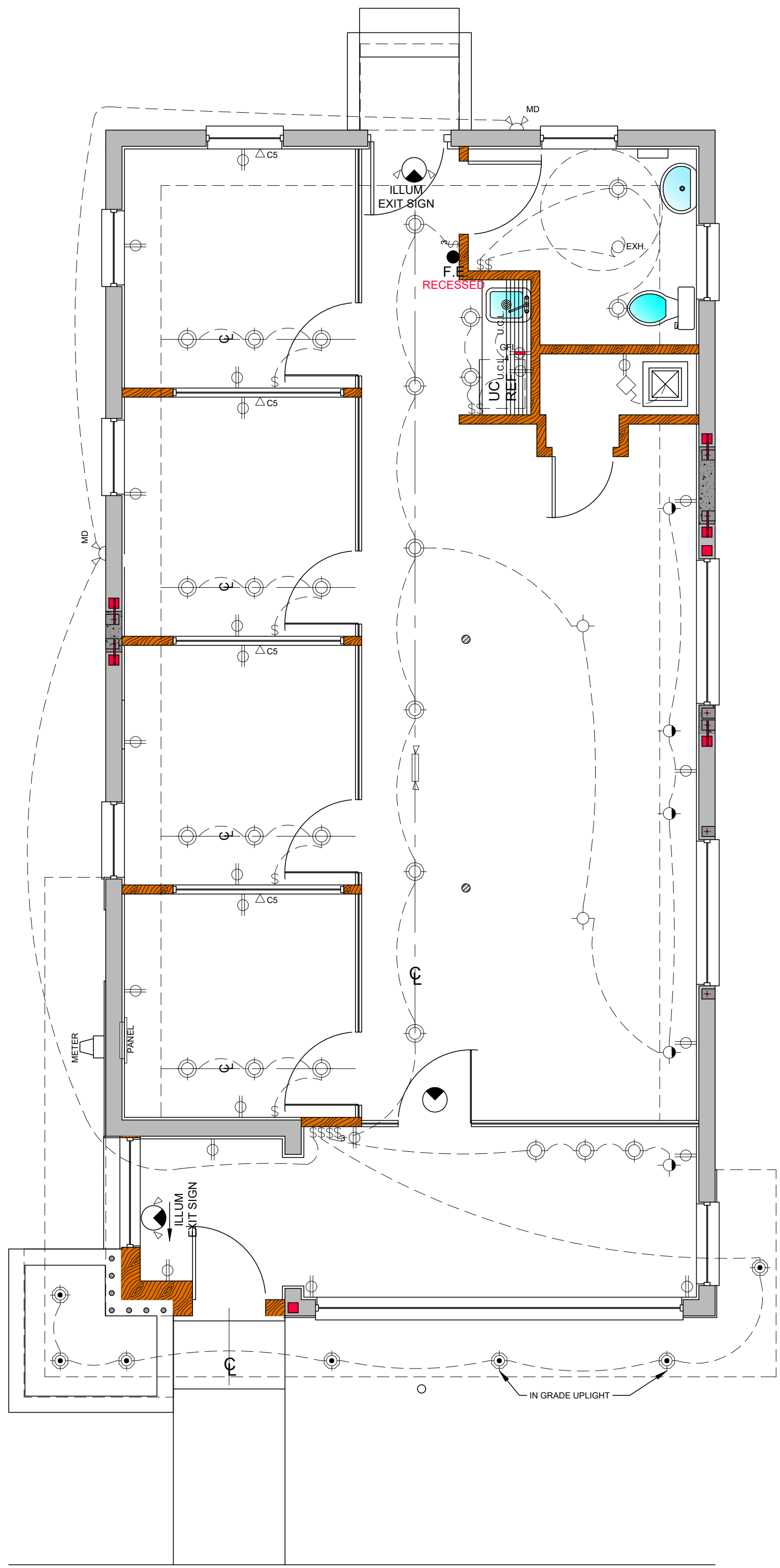
Electrical Floor Plan Scale: 1/4" = 1'-0"
