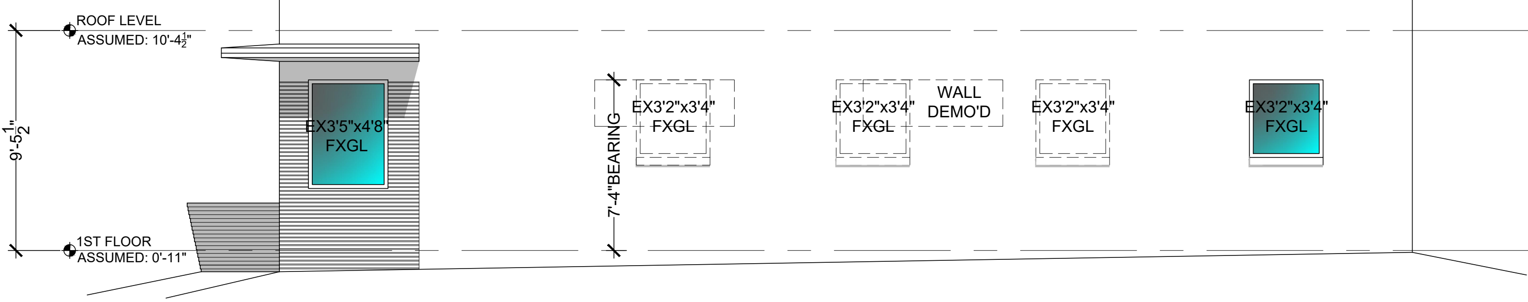
West Elevation Existing Scale: 1/4" = 1'-0"
