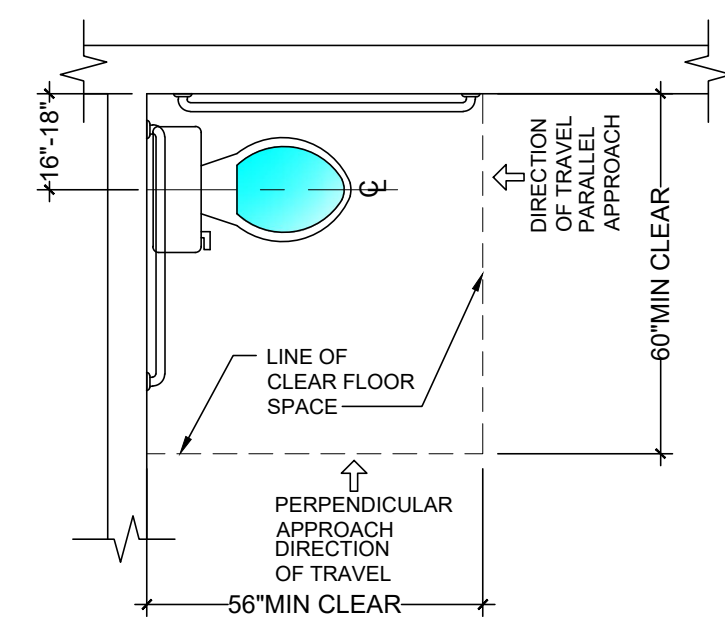
ADA Closet Clearances Scale: 3/8" = 1'-0"
