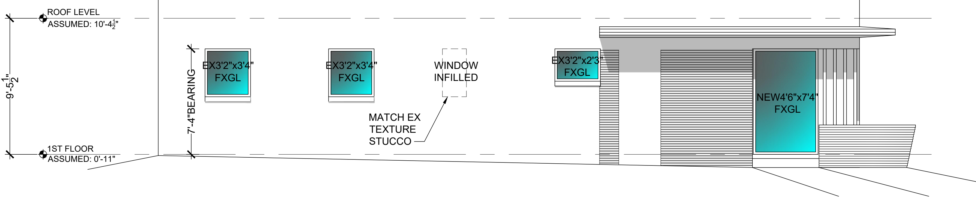
East Elevation Renovation Scale: 1/4" = 1'-0"
