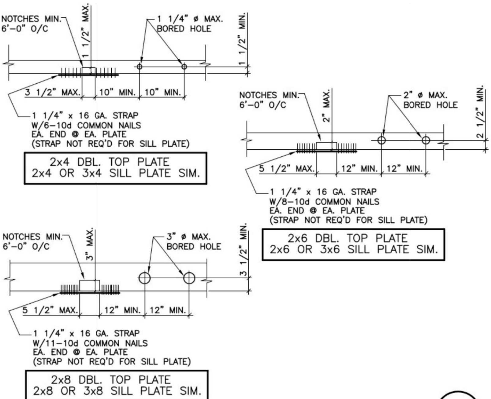
TYPICAL NOTCH & BORED TOP PLATE
