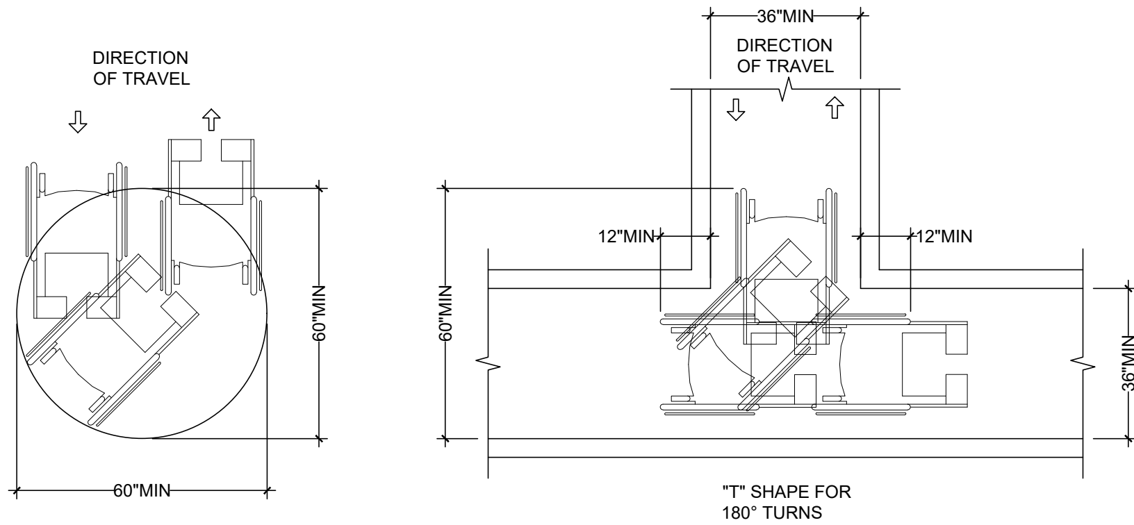
Accessible Turn Around Scale: 3/8" = 1'-0"
