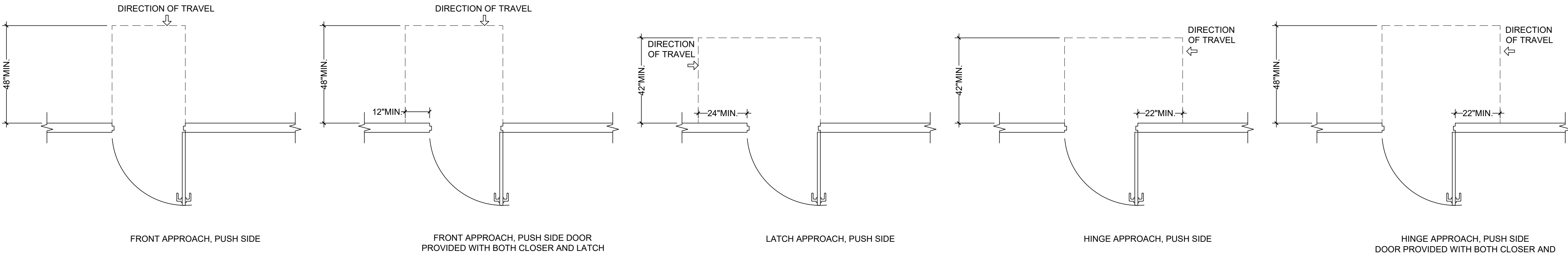
Maneuvering Clearance at Doors and Gates Scale: 3/8" = 1'-0"
