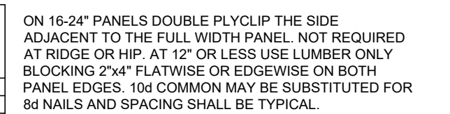
Typical Sheathing Nailing Schedule Scale: N.T.S.
