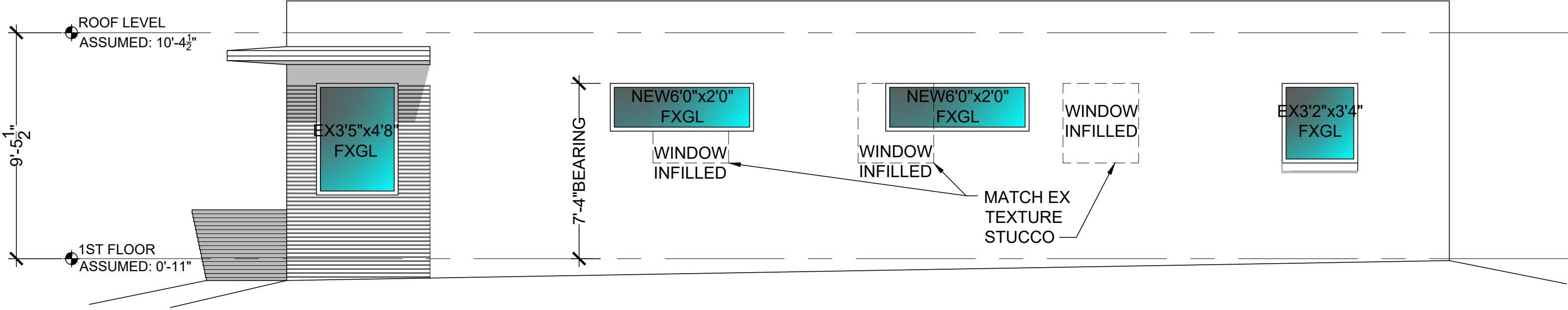
West Elevation Renovation Scale: 1/4" = 1'-0"
