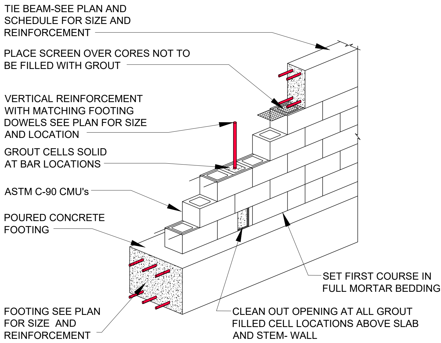
Typical Masonry Wall Construction Scale: 1/2"=1'-0"
